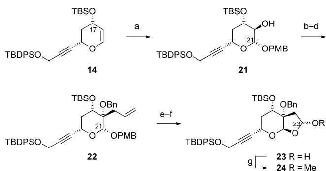
Scheme 6. Completion of the core for propargylic mesylate 2 : a) DMDO, acetone/CH 2 Cl 2 (1:1), 0°C; then PMBOH, ZnCl 2 , CH 2 Cl 2 , 0°C to RT, 86%; b) Dess–Martin periodinane, CH 2 Cl 2 , RT; c) (allyl)MgBr, THF, –110°C; d) NaH, BnBr, DMF, 0°C to RT, 52% (over 3 steps); e) O 3 , CH 2 Cl 2 , –78°C; then PS–PPh 3 , RT; f) CH 2 Cl 2 (90 ppm water)/TFA (9:1), RT; g) Amberlyst A-15, molecular sieves (3 Å), MeOH/MeCN (1:10), RT, 1:1 to 1:5 ( \alpha/\beta ) mixture of C23-epimers. PS = polystyrene supported.
