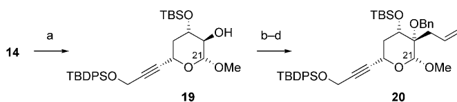
Scheme 5. Preparation of methyl acetal 20 for the synthesis of 2 : a) DMDO, acetone/CH 2 Cl 2 (1:1), 0°C; then MeOH, 82%; b) Dess–Martin periodinane, CH 2 Cl 2 , RT; c) (allyl)MgBr, THF, –78°C, 78% (over 2 steps); d) NaH, BnBr, DMF, 0°C to RT, 62%. DMDO = dimethyldioxirane, DMF = N,N -dimethylformamide, THF = tetrahydrofuran.
